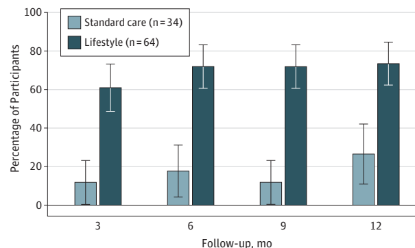
Figure 3. Proportion of Participants With Non-Insulin-Dependent Type 2 Diabetes With a Reduction in Glucose-Lowering Medication From Baseline in the Lifestyle vs Standard Care Groups
